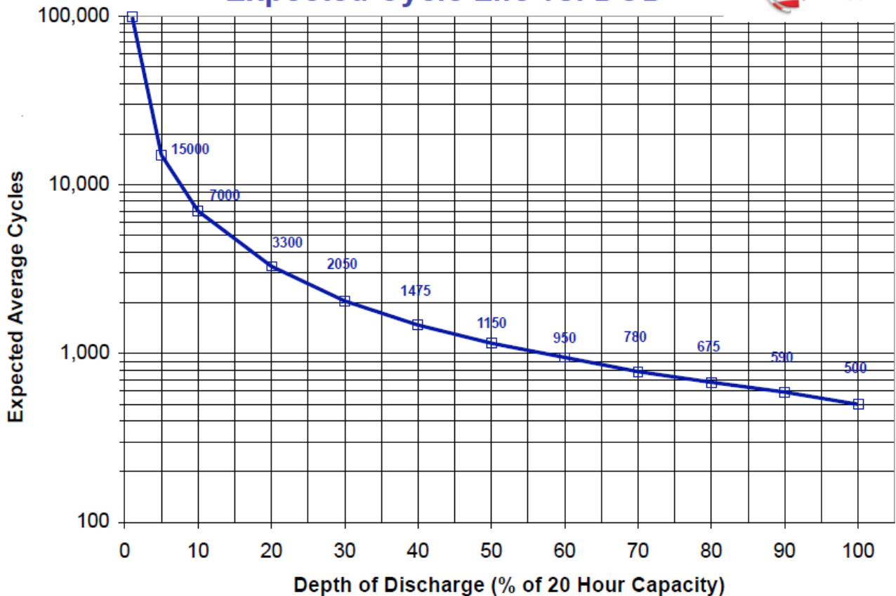
U. S Battery Manufacturing Co. Expected Cycle Life vs. DOD
